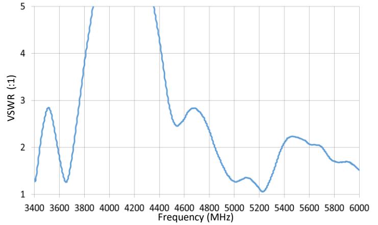
VSWR (3400 - 6000 MHz)
