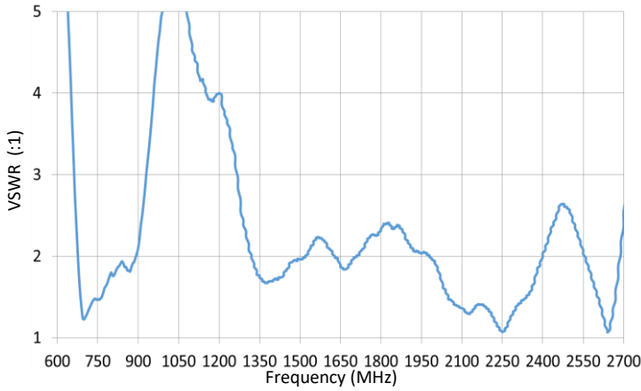
VSWR (600 - 2700 MHz)
