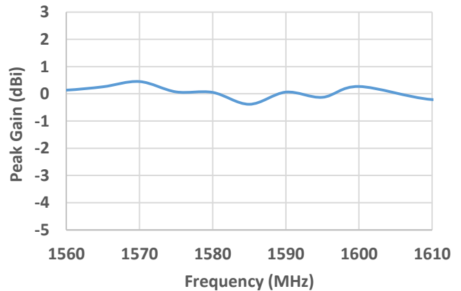
Peak Gain GNSS (1560 – 1610 MHz)
