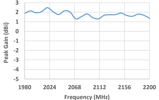
Peak Gain S-Band (1980 – 2200 MHz)
