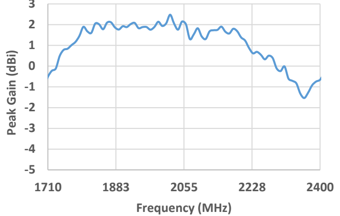
Peak Gain Mid Band (1710 – 2400 MHz)
