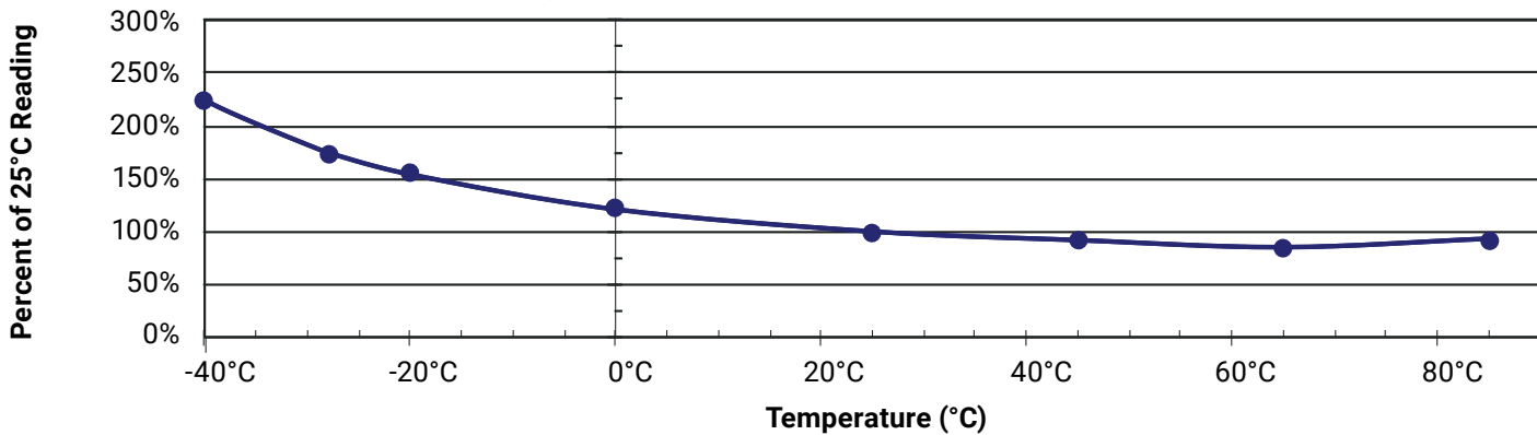
EQUIVALENT SERIES RESISTANCE VS. TEMPERATURE
