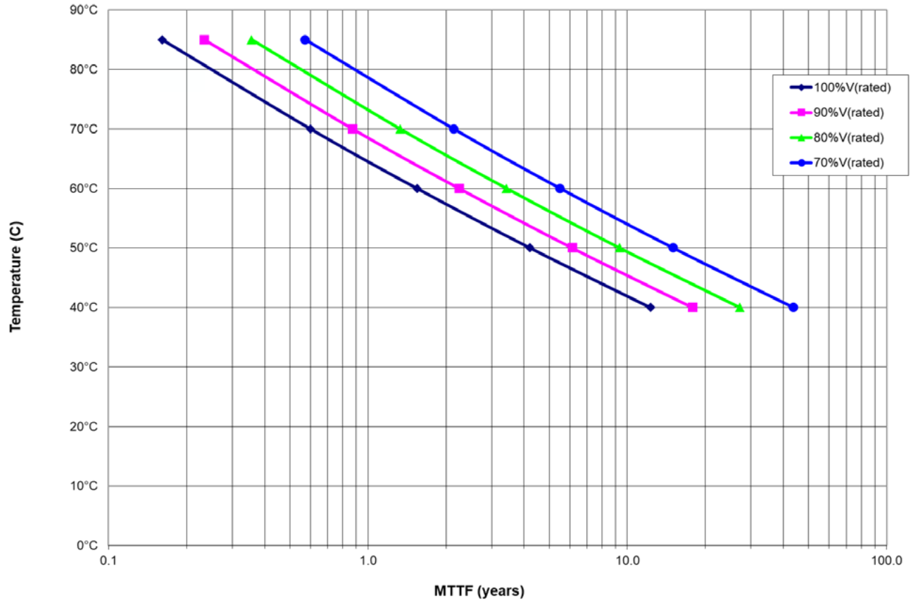
Expected Lifetime at Various Voltages SCC series
