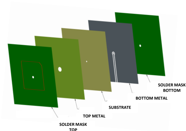
BOARD LAYOUT-01
