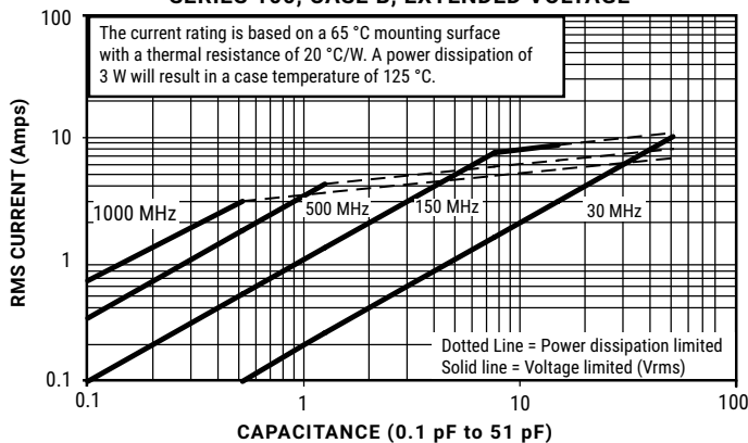
CURRENT RATING VS CAPACITANCE SERIES 100, CASE B, EXTENDED VOLTAGE
